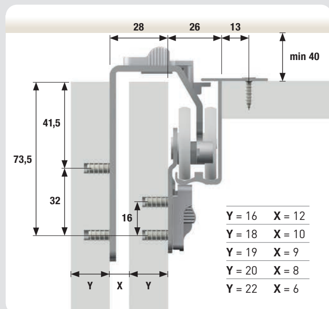
Carrelli superiori Upper rollers
